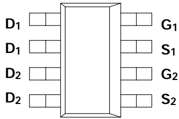
PARTMARKING DETAIL - M4206N
