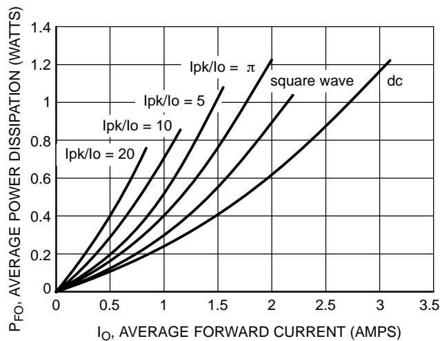
Figure 16. Forward Power Dissipation
