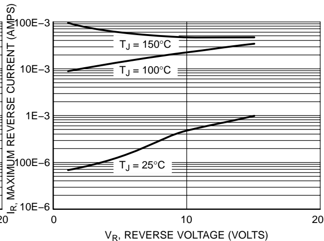
Figure 14. Maximum Reverse Current
