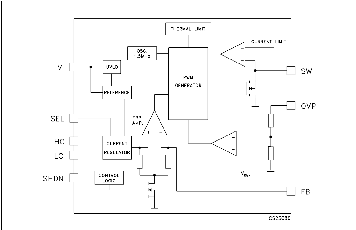
Figure 1. Block diagram
