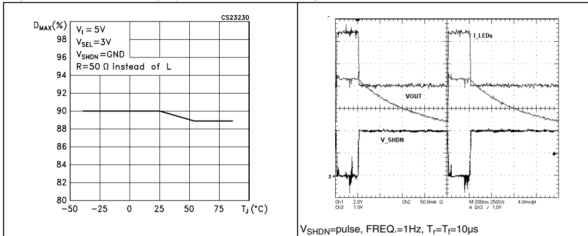
Figure 18. Turn on time
