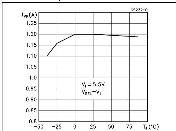
Figure 14. Peak inductor current vs temperature
