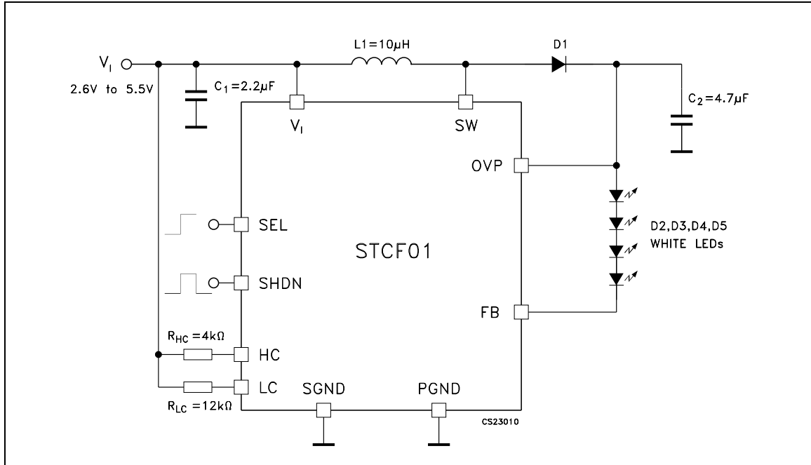
Figure 3. Application circuit
