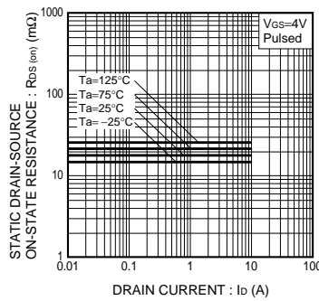
Fig.5 Static Drain-Source On-State Resistance vs. Drain Current(IV)
