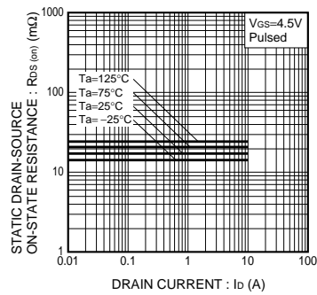
Fig.4 Static Drain-Source On-State Resistance vs. Drain Current(III)
