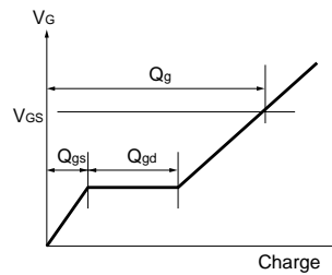
Fig.15 Gate Charge Waveform
