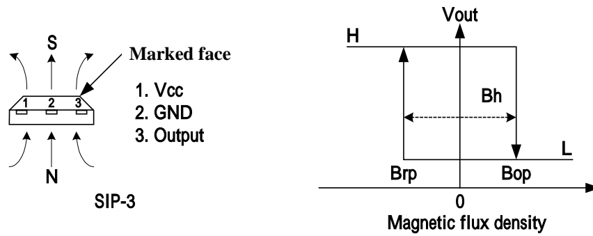
Fig. 2 APPLYING DIRECTION OF MAGNETIC FLUX
