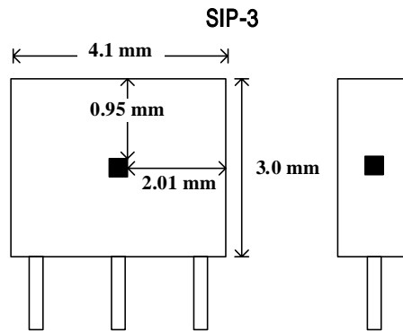
Fig. 1 SENSOR LOCATIONS
