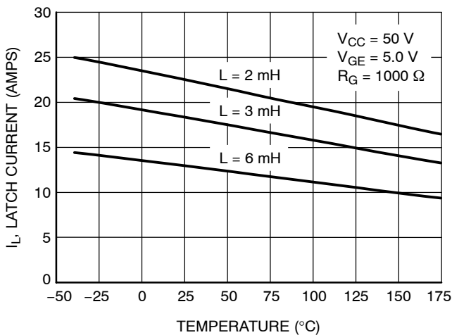
Figure 11. Typical Open Secondary Latch Current versus Temperature
