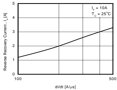
Figure 20. Typical Reverse Recovery Current
