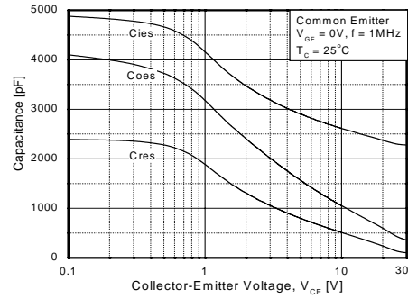
Figure 8. Capacitance Characteristics
