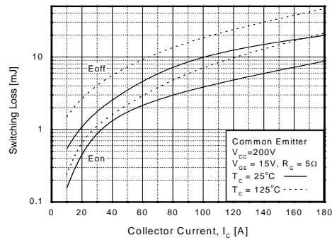
Figure 16. Switching Loss vs Collector Current
