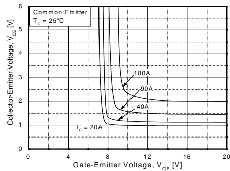
Figure 6. Saturation Voltage vs. V_{GE}
