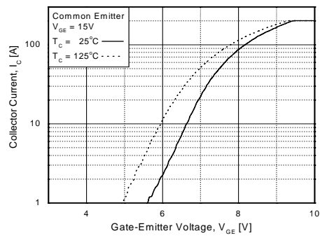
Figure 4. Transfer Characteristics
