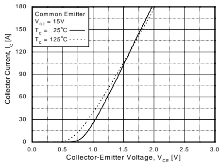
Figure 3. Saturation Voltage
