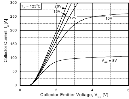
Figure 2. Typical Output Characteristics
