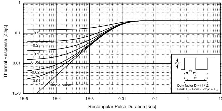
Figure 18. Transient Thermal Impedance of IGBT
