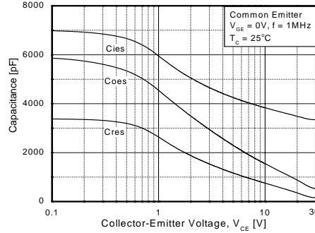
Figure 8. Capacitance Characteristics
