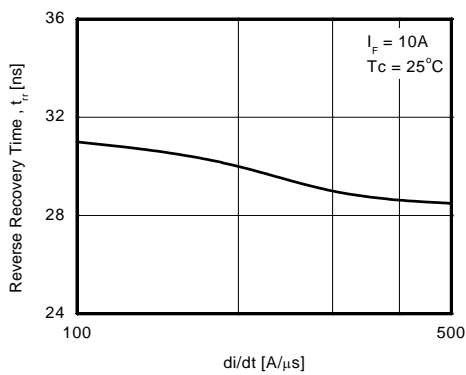
Figure 21. Typical Reverse Recovery Time
