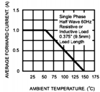
FIG.2- MAXIMUM AVERAGE FORWARD CURRENT DERATING
