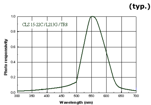
Fig.6 Spectral Response (Green region)
