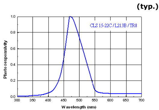
Fig.5 Spectral Response (Blue region)
