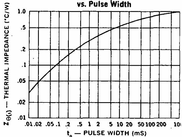
Thermal Impedance vs. Pulse Width
