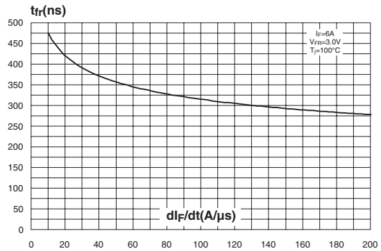
Figure 6: Forward recovery time versus di_F/dt (typical values)
