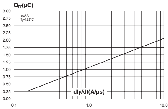
Figure 3: Reverse recovery charges versus di_F/dt (typical values)
