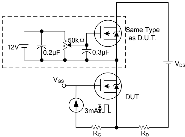
3A Gate Charge Test Circuit
