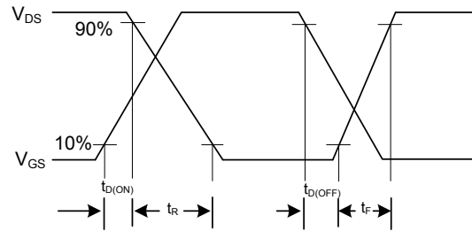
2B Switching Waveforms
