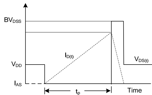
4B Unclamped Inductive Switching Waveforms
