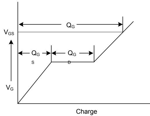
3B Gate Charge Waveform
