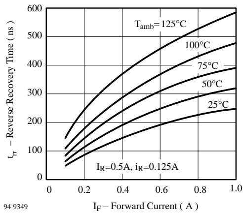
Figure 4. Max. Reverse Recovery Time vs. Forward Current
