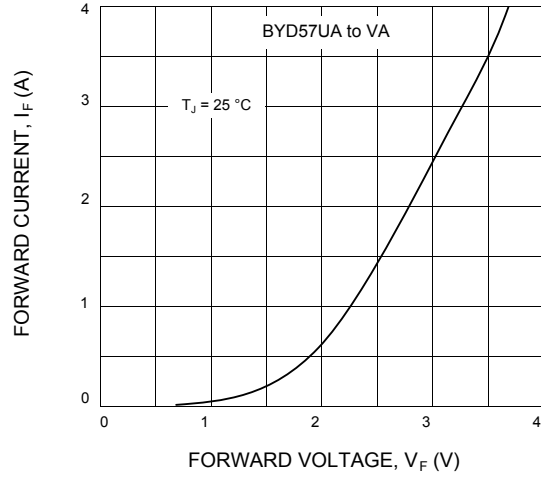
FIG.8 - FORWARD CURRENT AS FUNCTION OF FORWARD VOLTAGE
