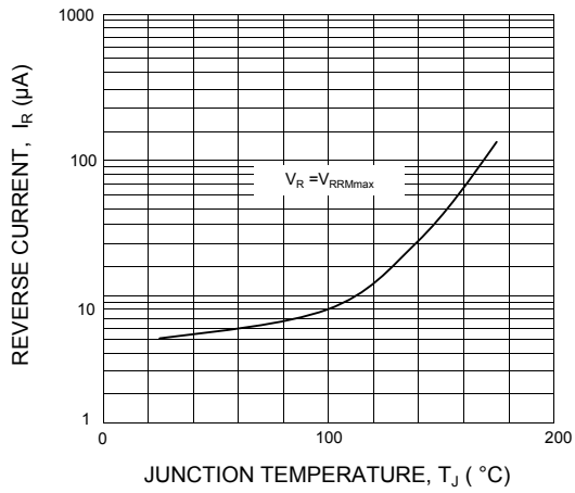
FIG.9 - REVERSE CURRENT AS FUNCTION OF JUNCTION TEMPERATURE
