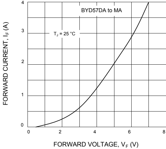
FIG.7 - FORWARD CURRENT AS FUNCTION OF FORWARD VOLTAGE
