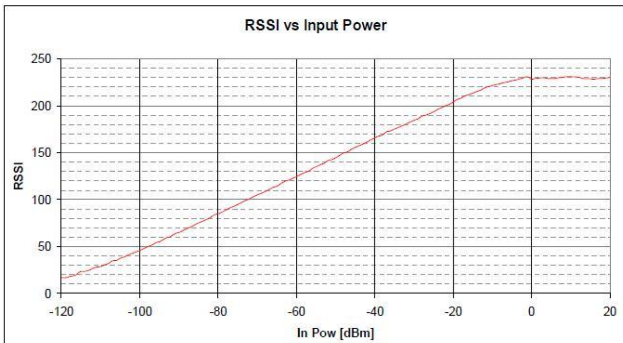
Figure 24. RSSI Value vs. Input Power
