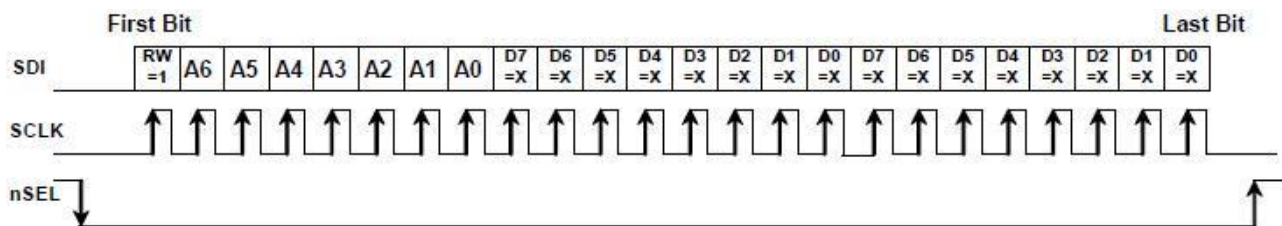
Figure 4. SPI Timing—Burst Write Mode
