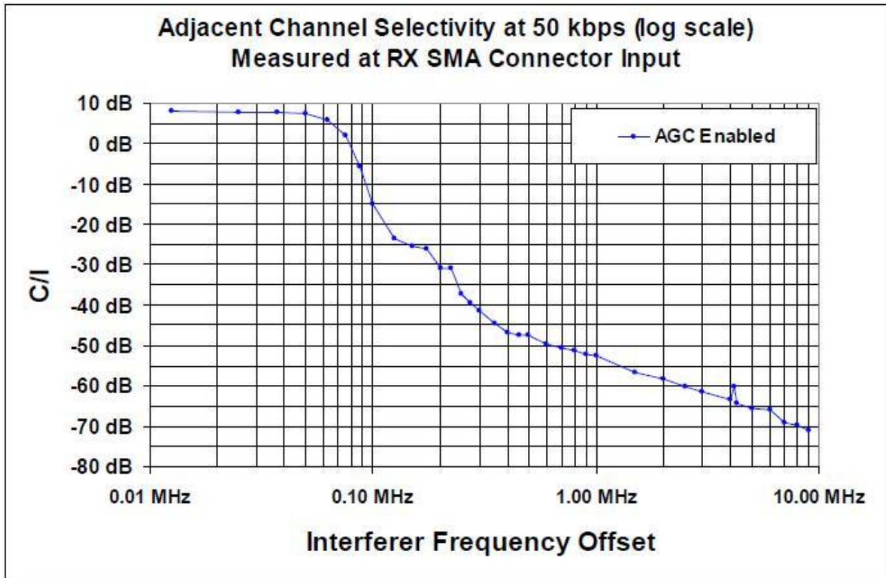
Figure 30. Receiver Selectivity
