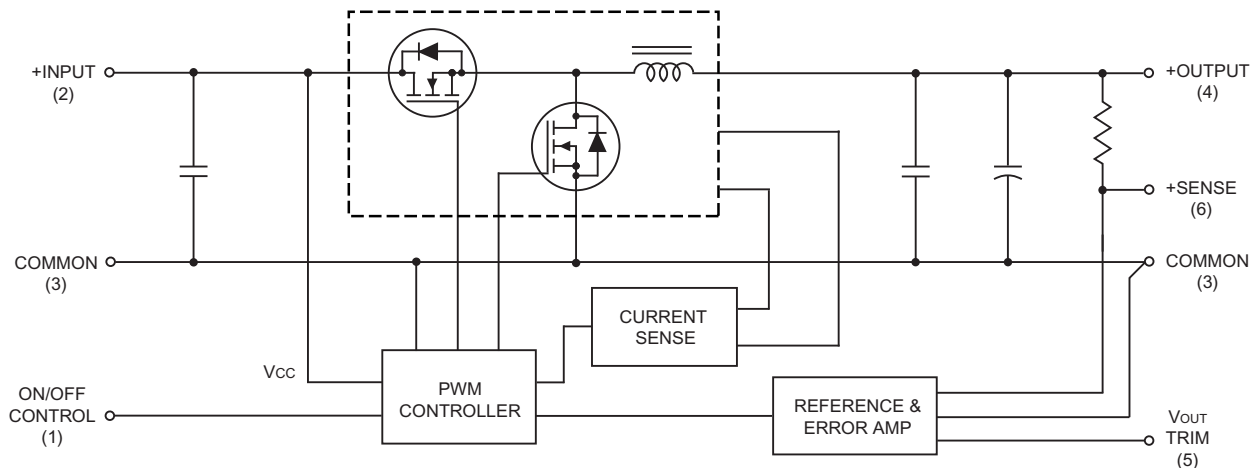
Figure 1. Simplified Schematic
