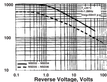
Fig. 3 - Typical Junction Capacitance
