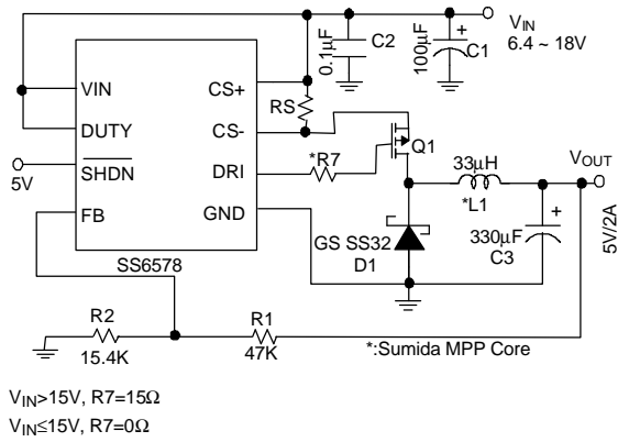
Fig. 7 5V Step-Down Converter
