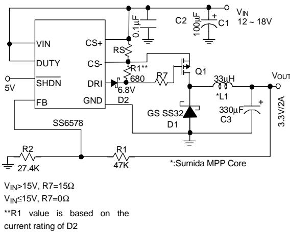
Fig. 8 3.3V Step-Down Converter
