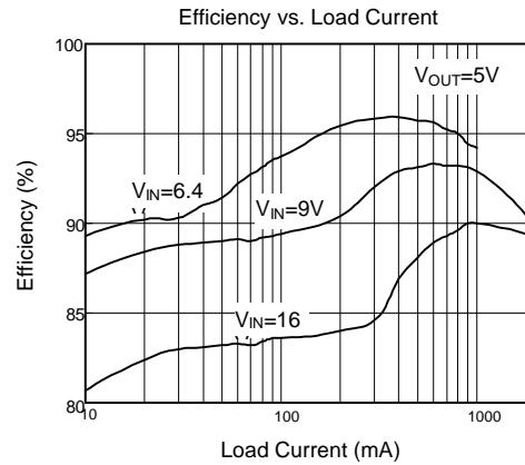
Fig. 7 5V Step-Down Converter
