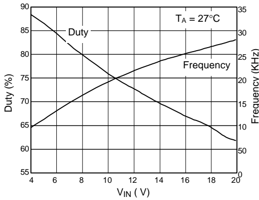
Fig. 1 Frequency & Duty Cycle vs. V_{IN}
