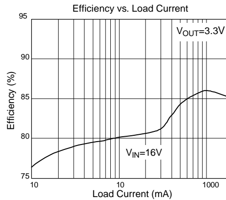
Fig. 8 3.3V Step-Down Converter
