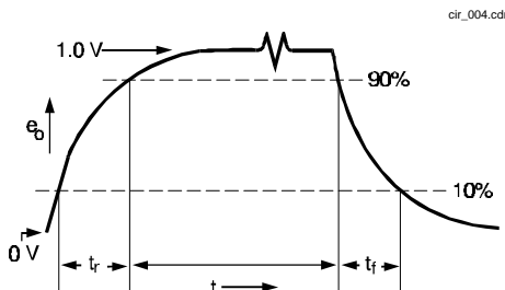
SWITCHING WAVEFORM
