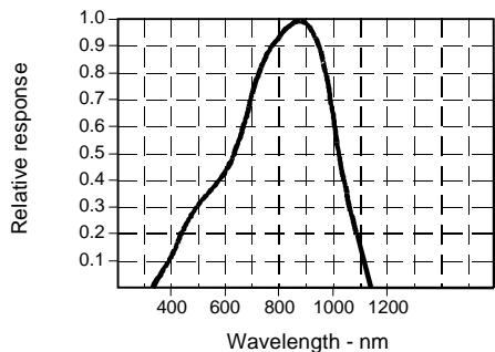
Fig. 5 Spectral Responsivity
