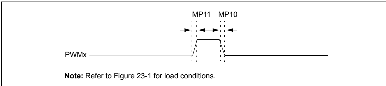
FIGURE 23-11: MOTOR CONTROL PWM MODULE TIMING CHARACTERISTICS
