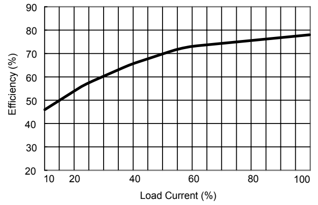
Figure 2: Efficiency vs. Output Load
