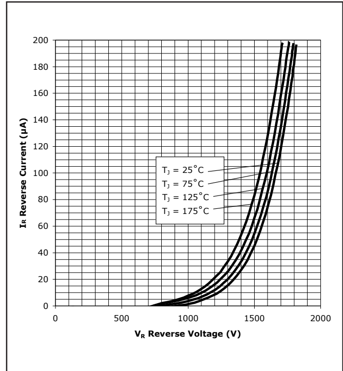
Figure 2. Reverse Characteristics
