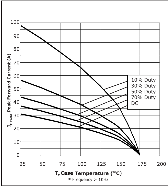
Figure 3. Current Derating
