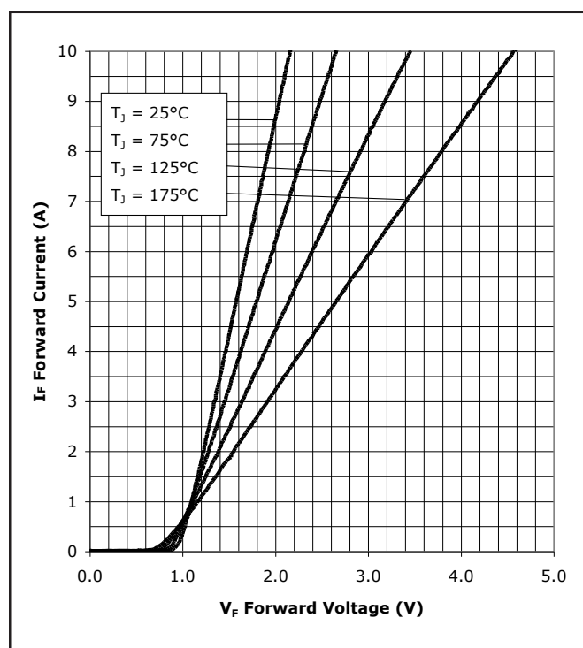
Figure 1. Forward Characteristics
