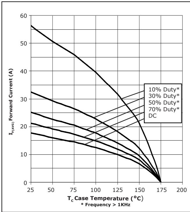
Figure 3. Current Derating
