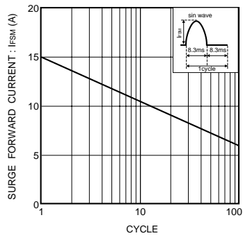
Fig.5 Forward peak surge current
