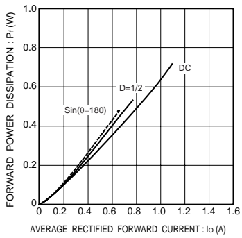
Fig.4 Power dissipation characteristics
