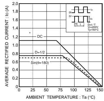
Fig.3 Derating curve
