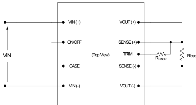
Figure D: Configuration for increasing output voltage.
