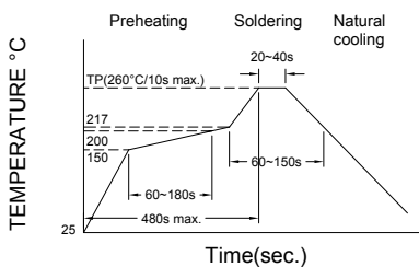
Figure 1. Re-flow Soldering
