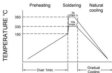
Figure 3. Hand Soldering
