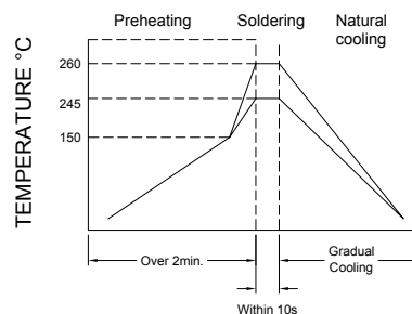
Figure 2. Wave Soldering
