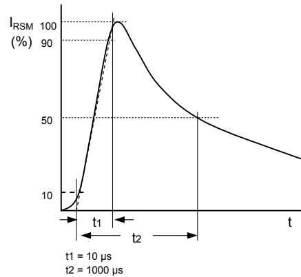
Fig.4 - Non-Repetitive peak reverse current pulse definition
