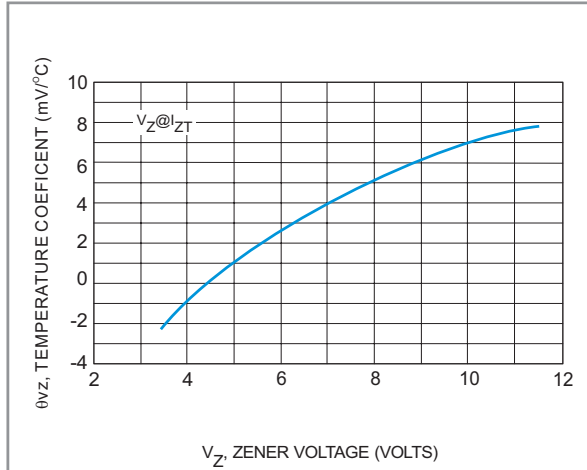
Fig.2 Zener Voltage - to 12 volts
