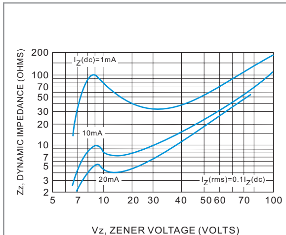
Fig.5 Effect of Zener Voltage
