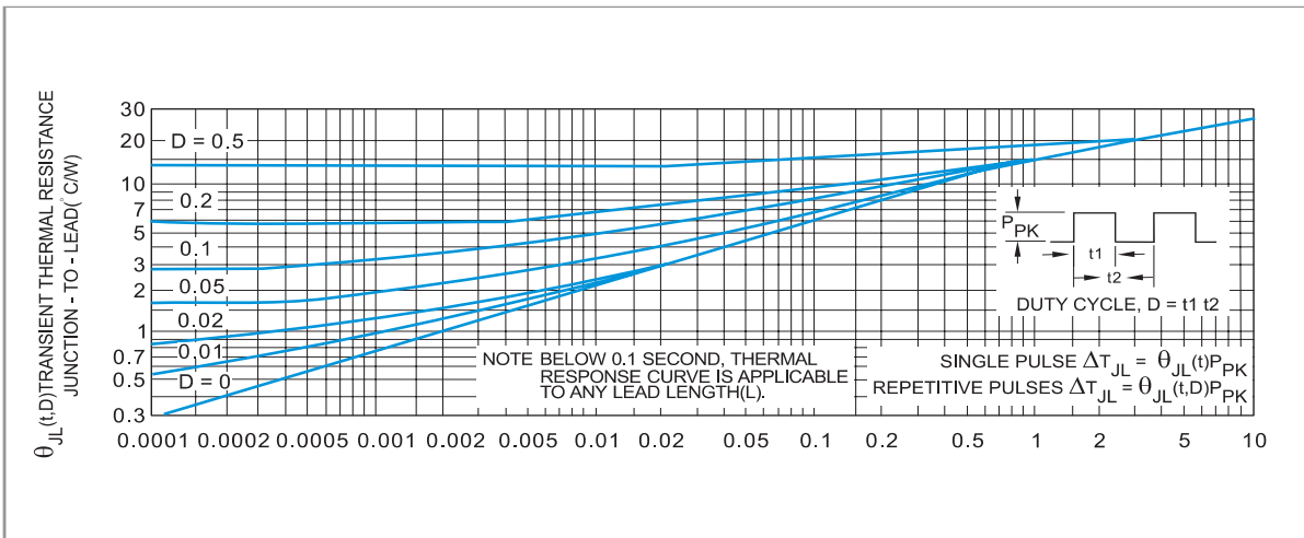
FIGURE 1. TYPICAL THERMAL RESPONSE L,
