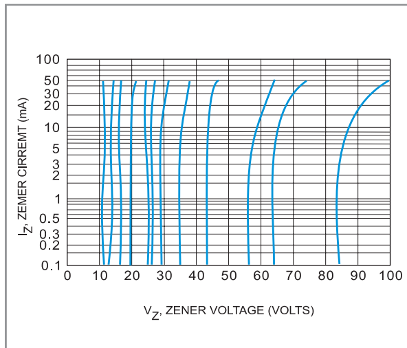
FIGURE 7 . V_Z = 12 THRU 82 VOLTS
