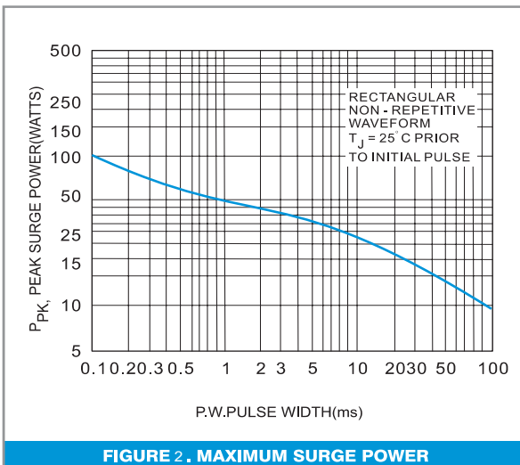
FIGURE 2. MAXIMUM SURGE POWER
