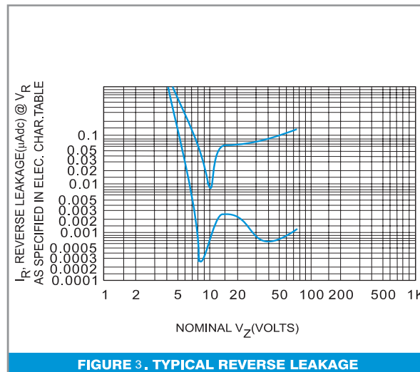
FIGURE 3. TYPICAL REVERSE LEAKAGE
