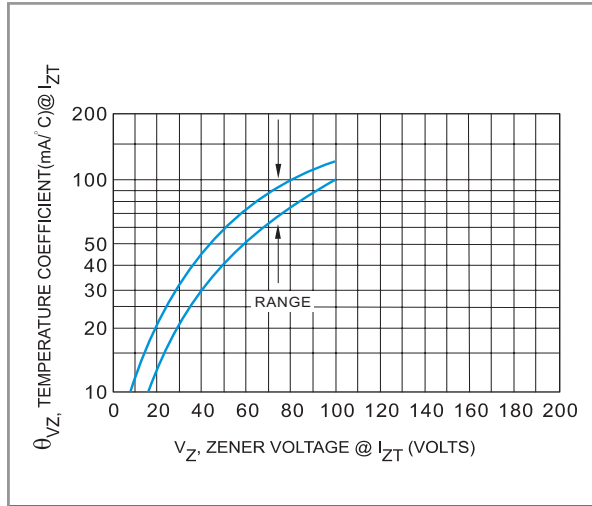
FIGURE 5 . UNIT 10 TO 200 VOLTS
