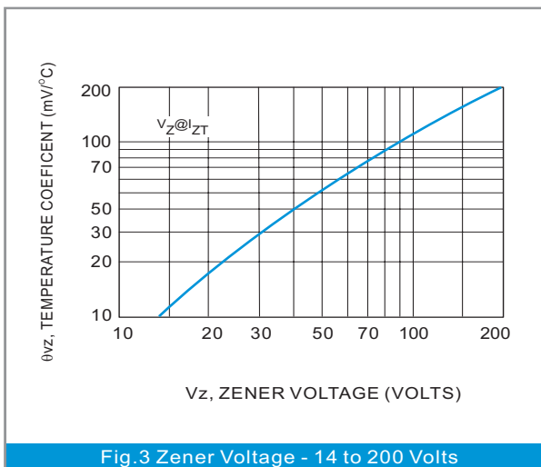
Fig.3 Zener Voltage - 14 to 200 Volts
