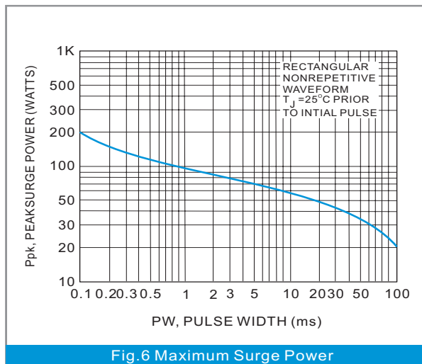
Fig.6 Maximum Surge Power
