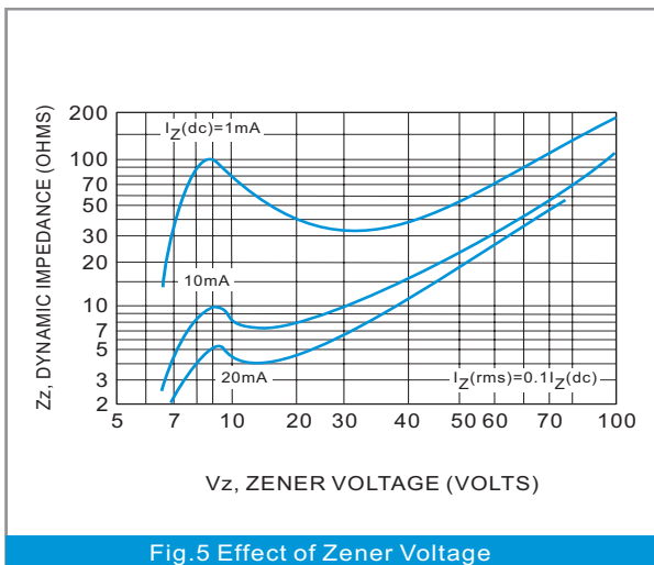
Fig.5 Effect of Zener Voltage
