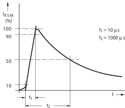
FIG.5 - Non-REPETITIVE PEAK REVERSE CURRENT PULSE DEFINITION
