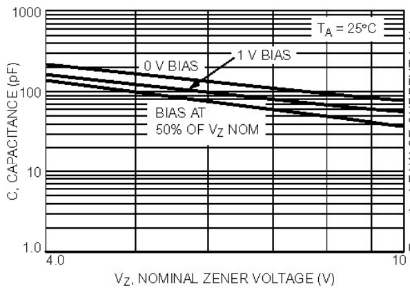
Figure 3. Typical Capacitance
