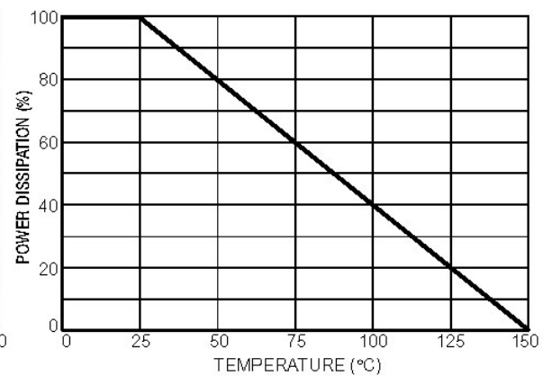
Figure 6. Steady State Power Derating
