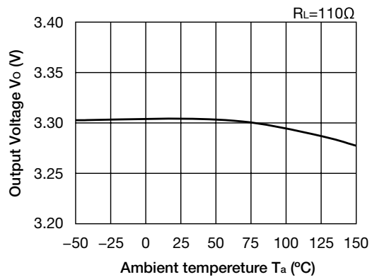
■ Output voltage - Ambient temperature
