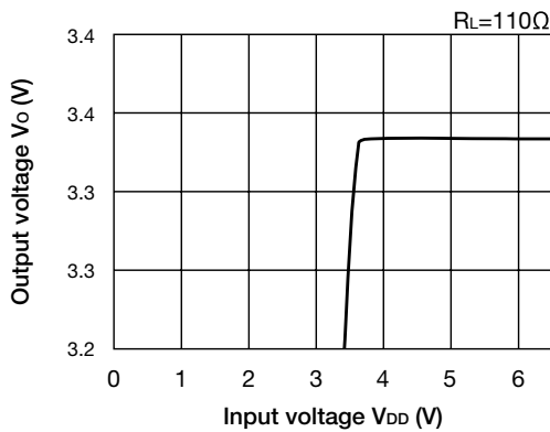
■ Line regulation
