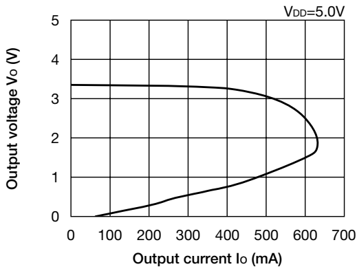
■ Output voltage - Output current
