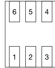
PLP-6A (TOP VIEW)
