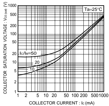
Fig.4 Collector-emitter saturation voltage vs. collector current ( II )
