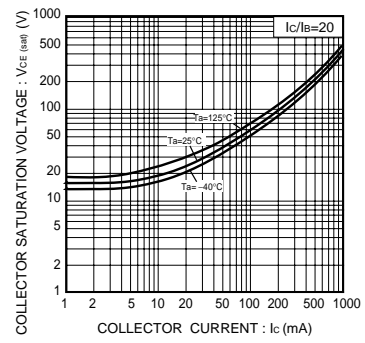
Fig.10 Collector-emitter saturation voltage vs. collector current (I)
