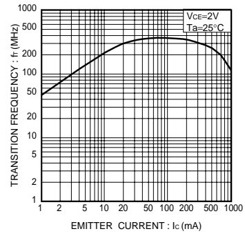
Fig.13 Gain bandwidth product vs. emitter current
