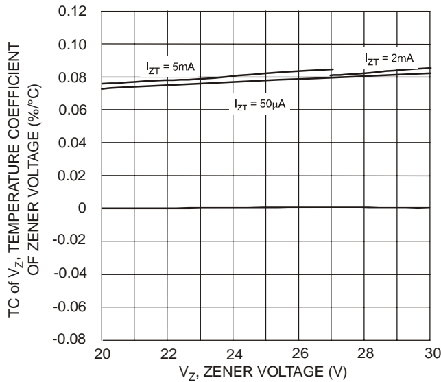
Fig. 18 Typical Temperature Coefficient of Zener Voltage, DDZX9707TS - DDZX9713TS
