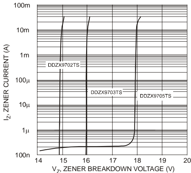
Fig. 6 Typical Reverse Characteristics, DDZX9702TS - DDZX9705TS
