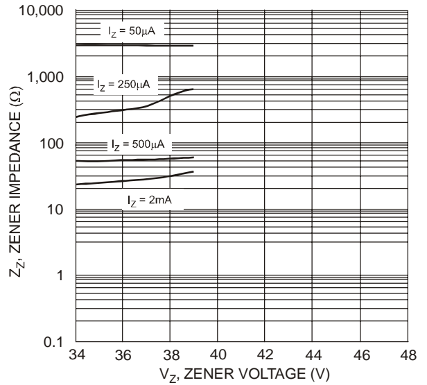
Fig. 15 Typical Zener Impedance Characteristics, DDZX9715TS - DDZX9717TS
