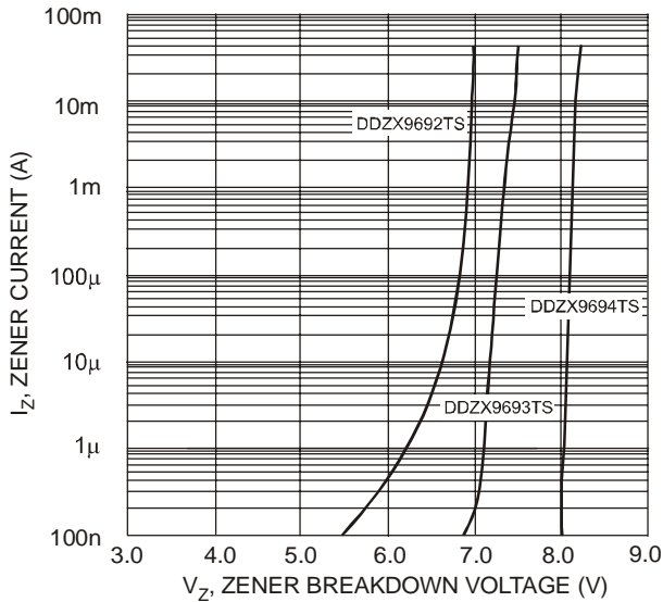
Fig. 4 Typical Reverse Characteristics, DDZX9692TS - DDZX9694TS
