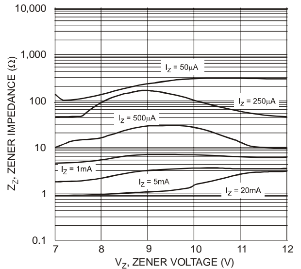
Fig. 11 Typical Zener Impedance Characteristics, DDZX9693TS - DDZX9699TS
