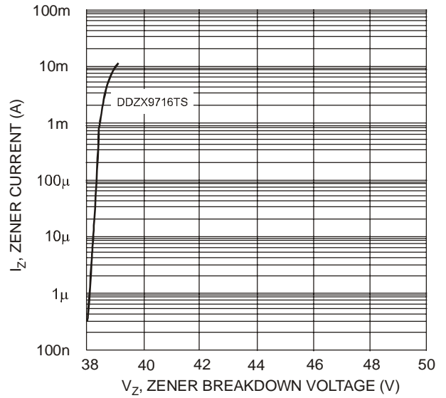
Fig. 9 Typical Reverse Characteristics, DDZX9716TS - DDZX9717TS
