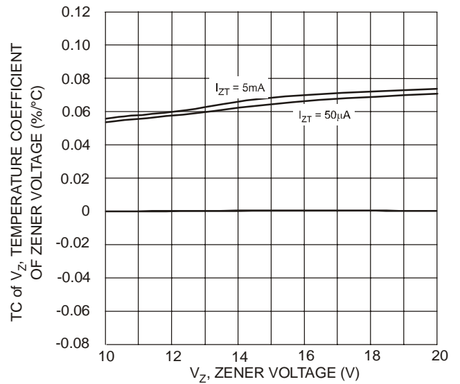
Fig. 17 Typical Temperature Coefficient of Zener Voltage vs. Zener Voltage, DDZX9697TS - DDZX9707TS
