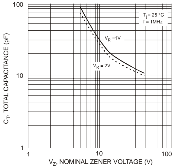
Fig. 20 Total Capacitance vs. Nominal Zener Voltage
