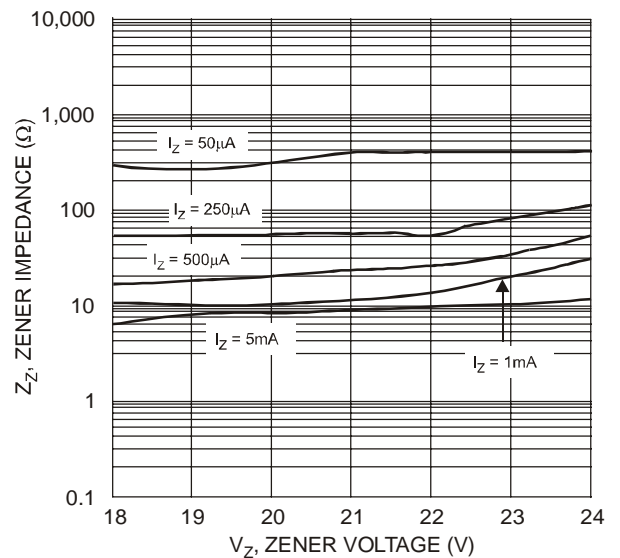
Fig. 13 Typical Zener Impedance Characteristics, DDZX9705TS - DDZX9709TS
