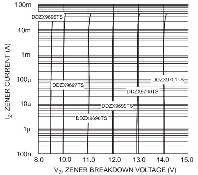
Fig. 5 Typical Reverse Characteristics, DDZX9696TS - DDZX9701TS
