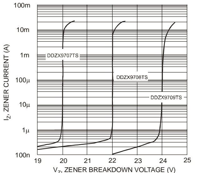
Fig. 7 Typical Reverse Characteristics, DDZX9707TS - DDZX9709TS
