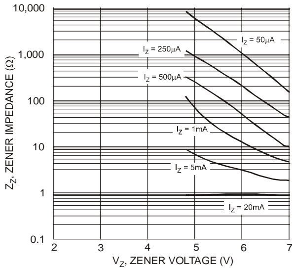
Fig. 10 Typical Zener Impedance Characteristics, DDZX9689TS - DDZX9692TS
