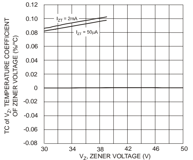
Fig. 19 Typical Temperature Coefficient of Zener Voltage, DDZ9713S - DDZ9716S
