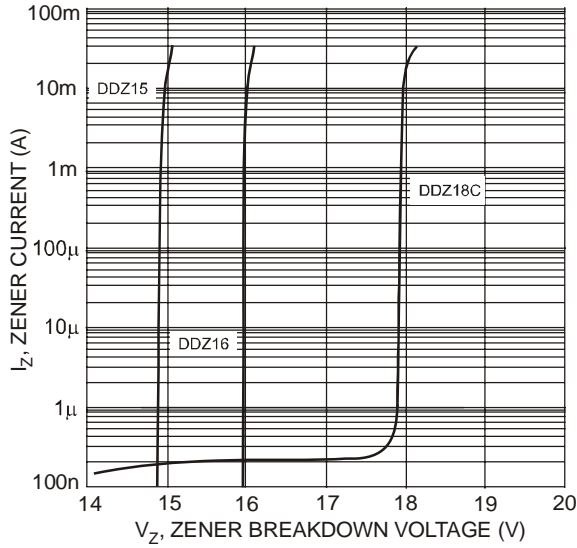
Fig. 6 Typical Reverse Characteristics, DDZ15 - DDZ18C
