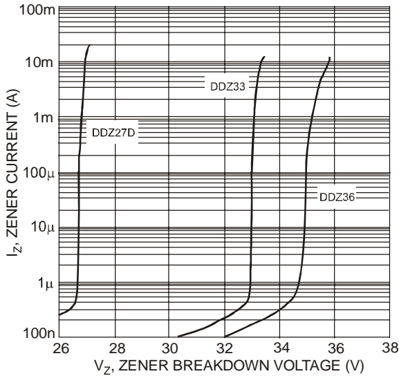
Fig. 8 Typical Reverse Characteristics, DDZ27D - DDZ36
