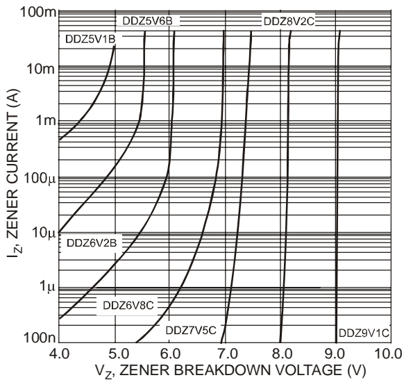
Fig. 4 Typical Reverse Characteristics, DDZ5V1B - DDZ9V1C
