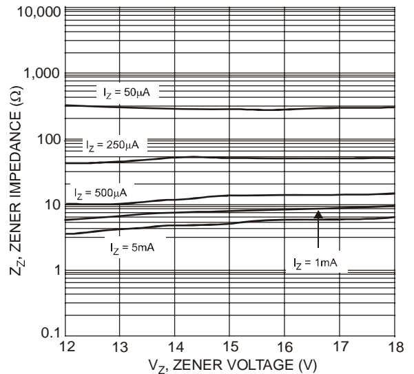
Fig. 11 Typical Zener Impedance Characteristics, DDZ12C - DDZ18C
