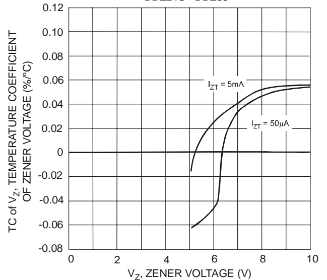
Fig. 15 Typical Temperature Coefficient of Zener Voltage vs. Zener Voltage, DDZ5V1B-DDZ10C
