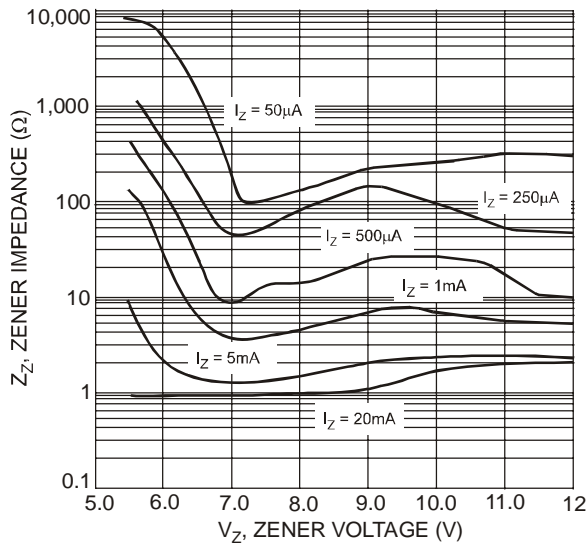
Fig. 10 Typical Zener Impedance Characteristics, DDZ5V6B - DDZ12C
