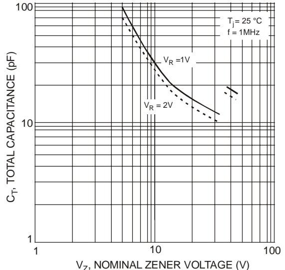
Fig. 19 Total Capacitance vs. Nominal Zener Voltage
