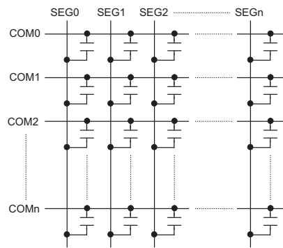
LCD Panel Equivalent Circuit
