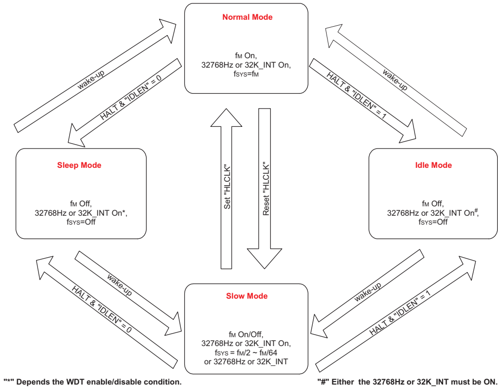
Dual Clock Mode Operation
