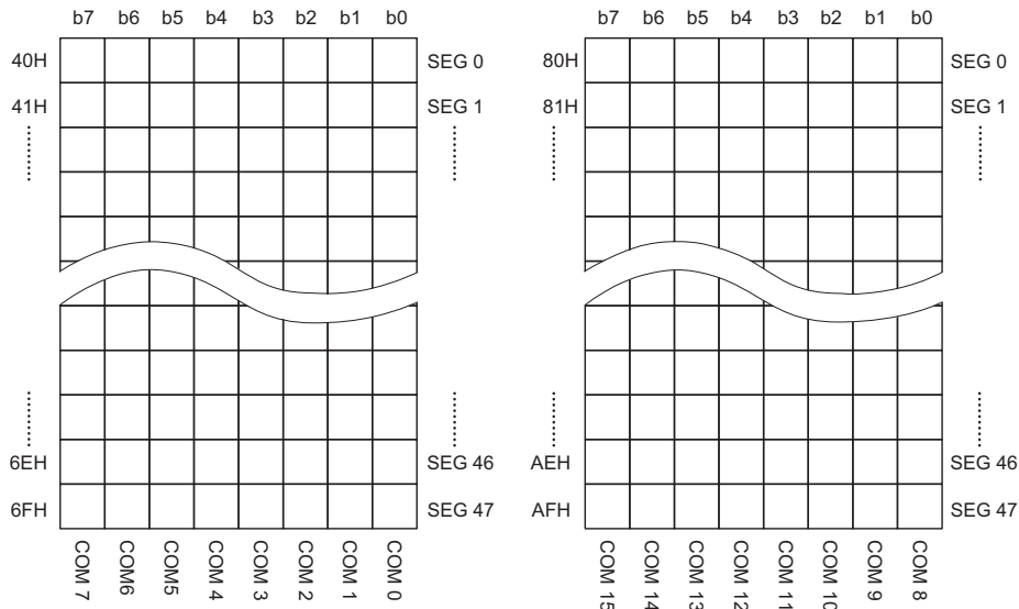
HT56R666 Memory Map – 48×16
