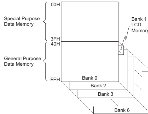
Data Memory Structure
