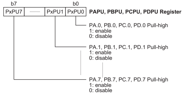
Pull-High Resistor Register – PAPU, PBPU, PCPU, PDPU
