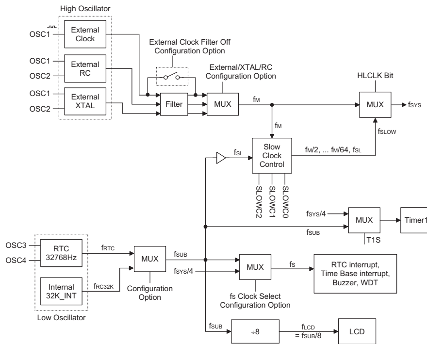
Dual Clock Mode Structure
