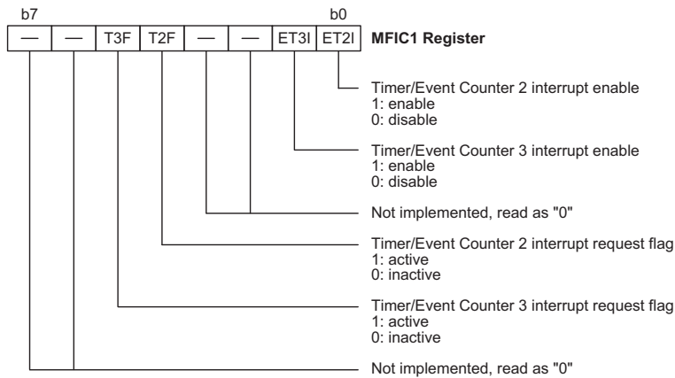
Interrupt Control Register – MFIC1
