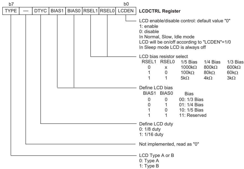
LCD Control Register – LCDCTRL - HT56R666
