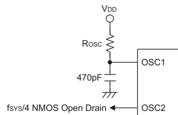
RC Oscillator
