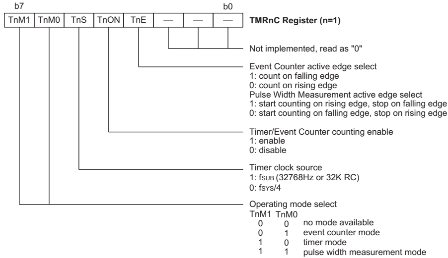
Timer/Event Counter Control Register – TMRnC
