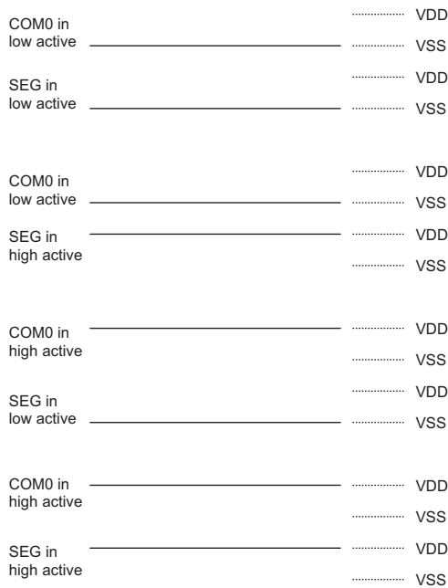
LED Static Mode Normal Operation
