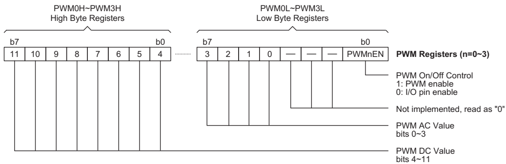
PWM Register Pairs
