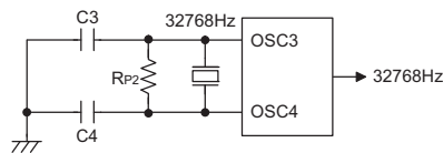
External 32768Hz Oscillator
