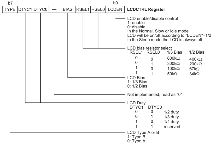
LCD Control Register – LCDCTRL - HT56R66
