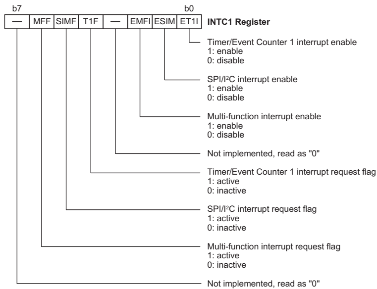
Interrupt Control Register – INTC1
