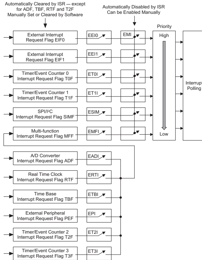
Interrupt Structure
