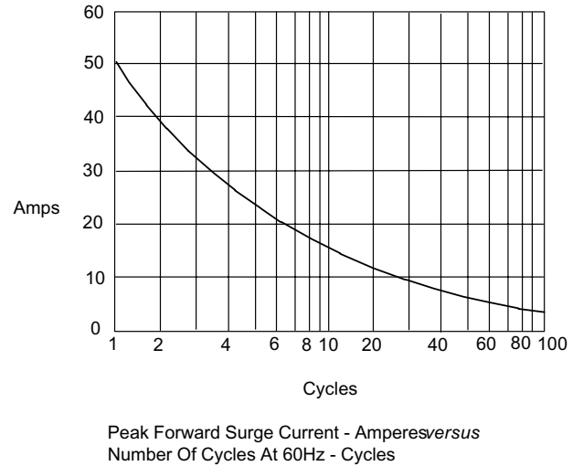
Figure 4 Maximum Non-Repetitive Forward Surge Current
