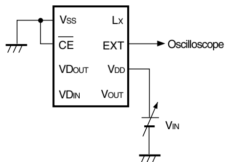
Test Circuit 3
