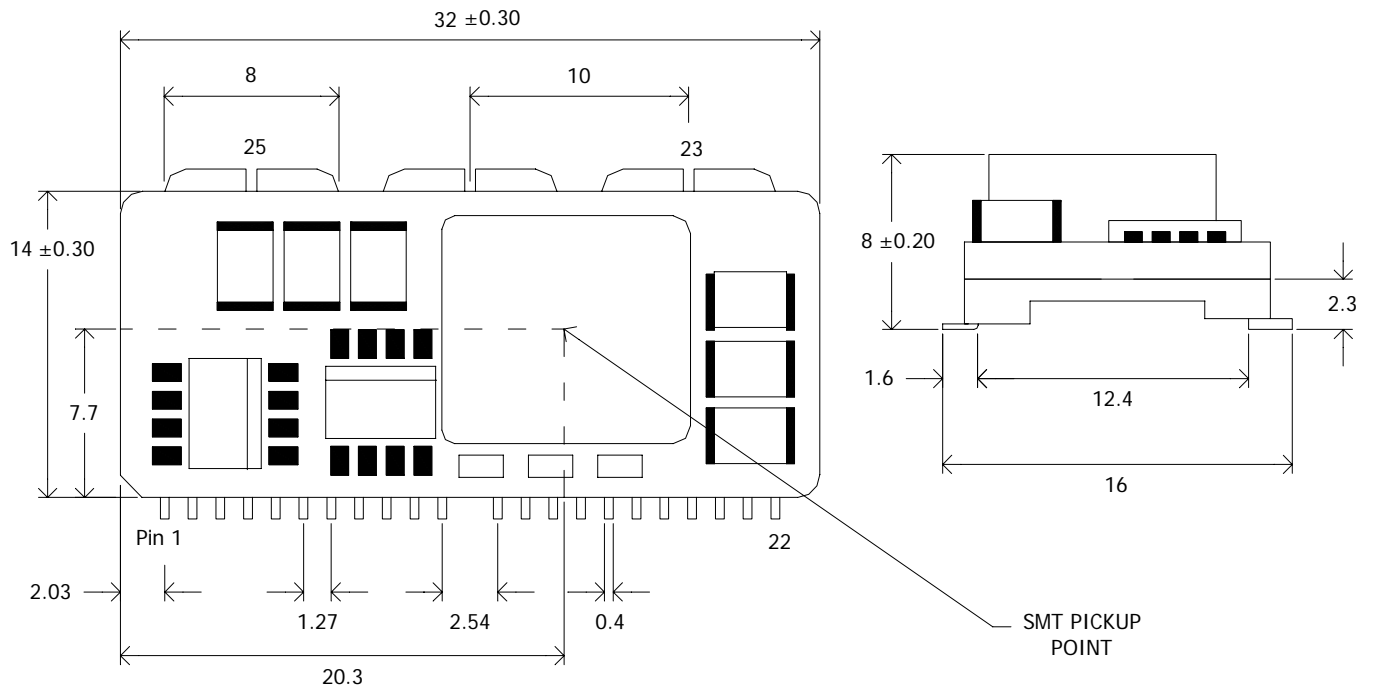
Figure 20. Mechanical Drawing
