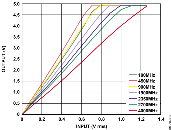
Figure 5. Output vs. Input Level (Linear Scale); Frequencies 100 MHz, 450 MHz, 900 MHz, 1900 MHz, 2350 MHz, 2700 MHz, and 4000 MHz; Supply 5.0 V
