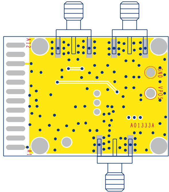
Figure 60. Layout of Evaluation Board, Circuit Side
