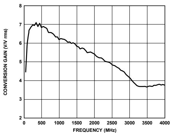
Figure 36. Conversion Gain vs. Frequency, Supply 5 V
