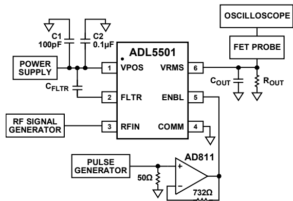
Figure 34. Hardware Configuration for Output Response to Enable Gating Measurements
