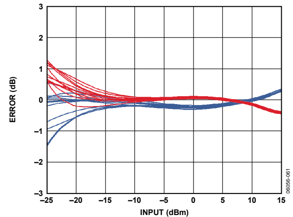
Figure 56. Temperature Drift Distributions for 12 Devices at -40^{\circ}\text{C} , +25^{\circ}\text{C} , and +85^{\circ}\text{C} After Ambient Normalization, Frequency 5.0 GHz, Supply 5.0 V
