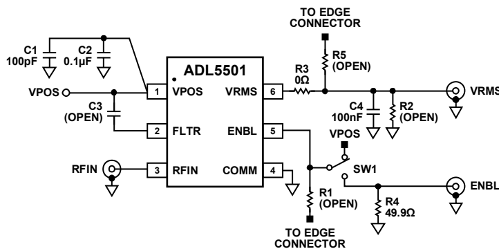
Figure 58. Evaluation Board Schematic
