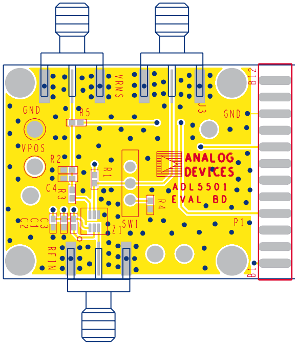
Figure 59. Layout of Evaluation Board, Component Side
