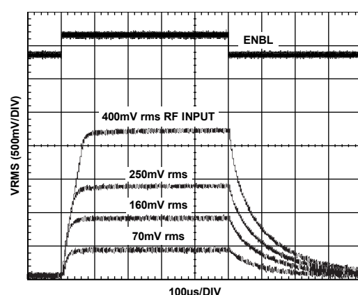
Figure 38. Output Response to Enable Gating at Various RF Input Levels, Supply 3 V, Frequency 900 MHz, C_{FLTR} = \text{Open} , C_{OUT} = 0.1\text{ μF} , R_{OUT} = 1\text{ kΩ}
