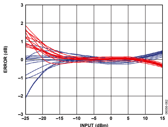
Figure 57. Temperature Drift Distributions for 12 Devices at -40^{\circ}\text{C} , +25^{\circ}\text{C} , and +85^{\circ}\text{C} After Ambient Normalization, Frequency 6.0 GHz, Supply 5.0 V
