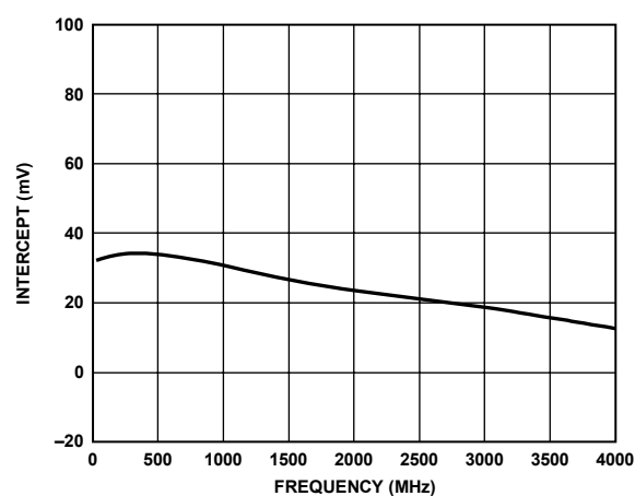
Figure 39. Intercept vs. Frequency, Supply 5 V
