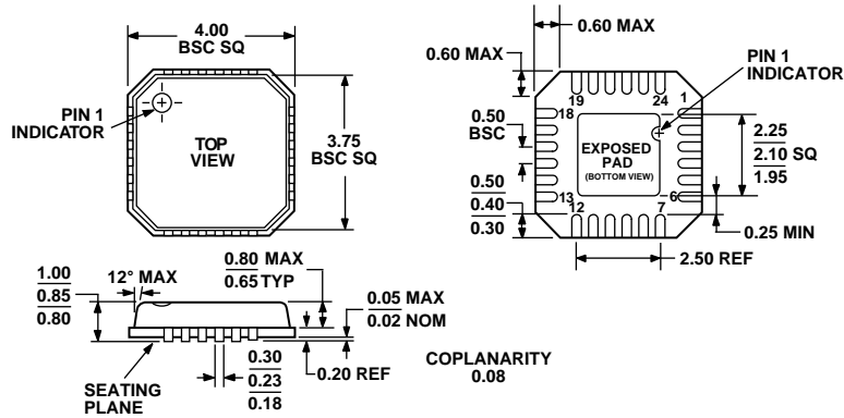
Figure 43. 24-Lead Lead Frame Chip Scale Package [LFCS] 4 mm x 4 mm Body (CP-24-1) Dimensions shown in millimeters
