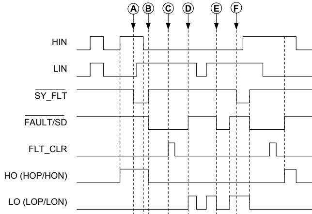
Figure 17: I/O Timing Diagram with SY_FLT and FAULT/SD as Output
