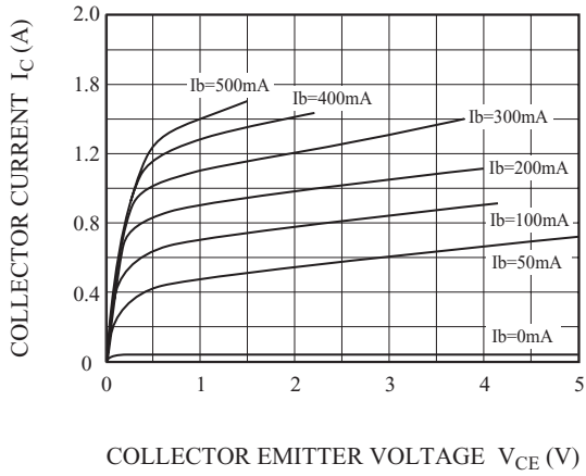
STATIC CHARACTERISTIC
