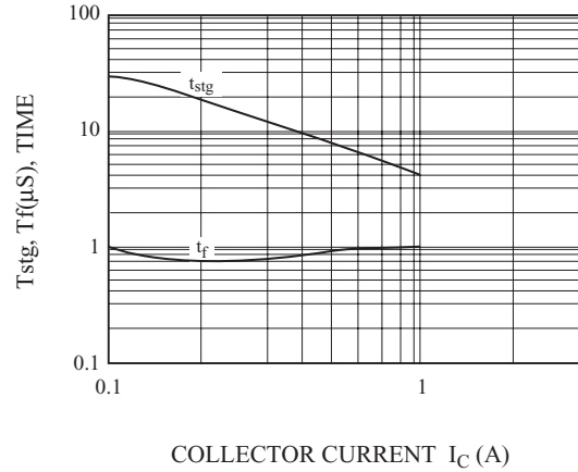
SWITCHING TIME
