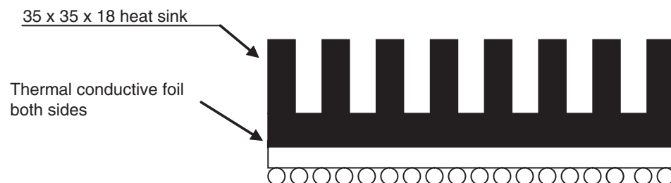
Figure 6-3. EV10AS150A-EB Evaluation Board Heat Sink Outlines
