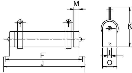
Non-Inductive Wirewound (DR-AN) G - Horizontal mount Dimensions
