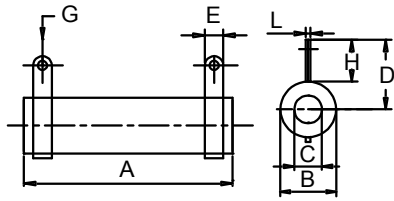
Round-Wirewound Power Resistor (DR-A) N - No mount Dimensions
