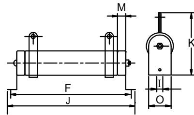
Round-Wirewound Power Resistor (DR-A) G - Horizontal mount Dimensions
