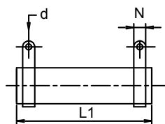
Non-Inductive Power Resistors (DR-BN) N - No mount Dimensions
