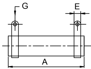
Non-Inductive Wirewound (DR-AN) N - No mount Dimensions
