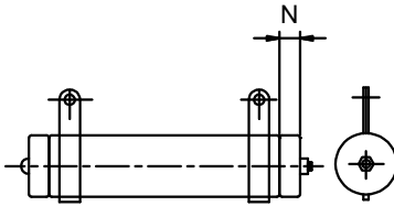
Round-Wirewound Power Resistor (DR-A) Z - Vertical mount Dimensions
