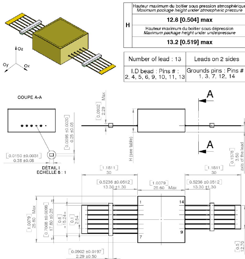
Figure 1 : Oscillator outline 1
