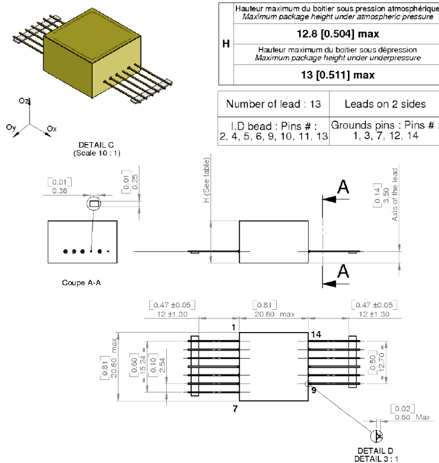
Figure 1 : Oscillator outline 1
